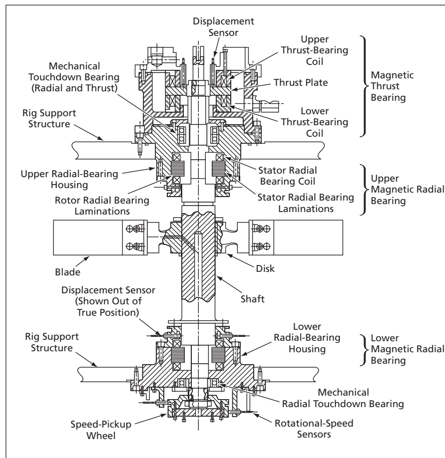
The Five-Axis, Three-Magnetic-Bearing configuration of this dynamic spin rig makes it possible to excite high-order vibrational modes of the disk-and-blade assembly. The five axes are the vertical thrust axis of the thrust bearing and two mutually perpendicular horizontal force axes for each of the two radial bearings.
