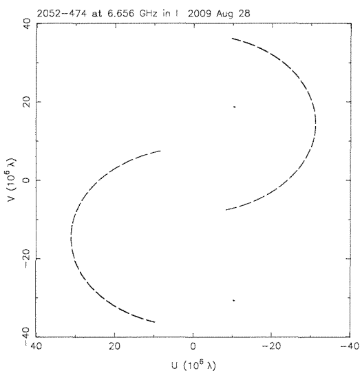
Fig. 4 The (u, v) coverage obtained from a 12 hour CHI observation of 2052-474. This is typical of a CHI experiment.
