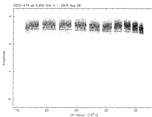
Fig. 6 Amplitude vs (u, v) distance plot of the calibrated 2052-474 CHI data. A model with major axis of 0.8 mas and an axial ratio of 1 well constrains the visibilities, giving an upper limit on the angular size of the source.
