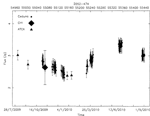
Fig. 5 Single dish and ATCA monitoring data of PKS 2052–474 overlaid with the CHI observation (the large filled diamond). The Ceduna data are the circles and the ATCA data the triangles. The VLBI data is consistent with both the single dish and the ATCA monitoring flux density. Note that the ATCA data are interpolated between simultaneous 5.5 and 9 GHz data to match the 6.7 GHz Ceduna single dish data.
