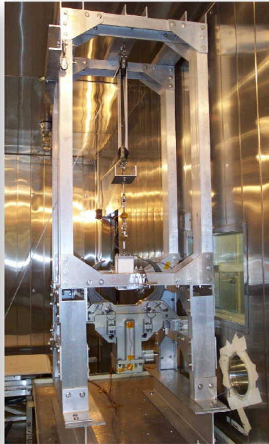
External Stowage Platform Attachment Device – Chamber H
