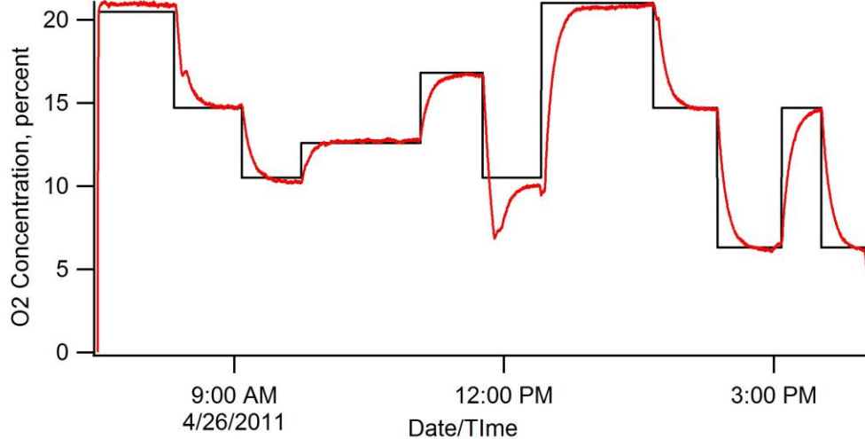
Fig 5. An example of a time-series data set obtained by acquiring the OLGA oxygen signal over about 8 hours on 04/26/2011. Black trace: feed concentration; red trace: OLGA measured [O 2 ].
