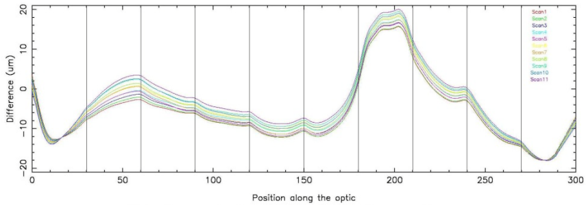
Distortion created by addition of the piezos – Power on
