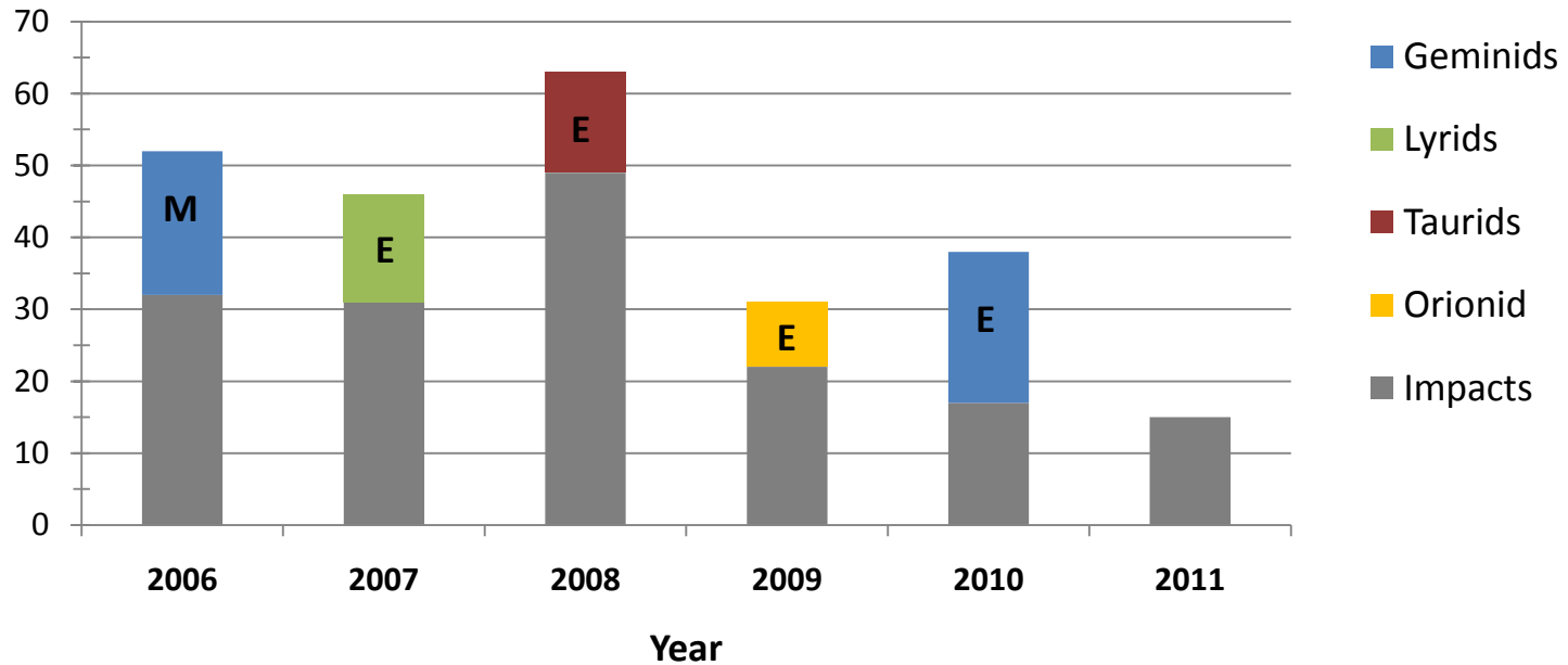
Observed Lunar Impacts 2006 -2011
