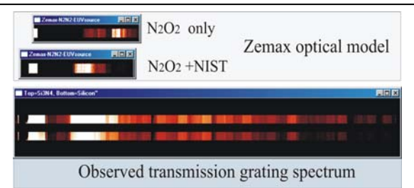
Figure 18. Zemax model (top images) with transmission grating observations using N 2 /O 2 . The top Zemax image assumes a perfect transmission grating with no absorption losses, the bottom image includes the NIST transmission measurements (Figure 15).
