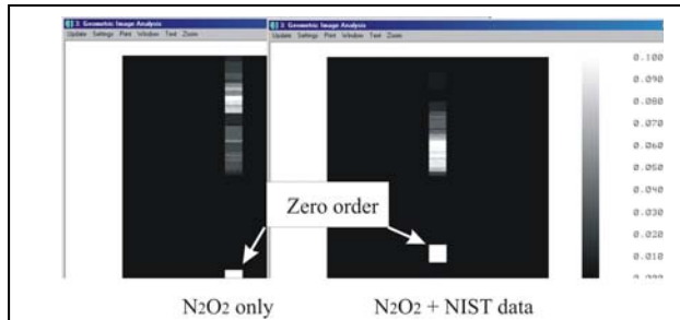
Figure 17. Zemax model of N 2 /O 2 spectrum with and without the NIST transmission data. This shows the inherent problem of determining the plate scale using just the observed spectrum.
