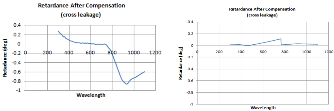
Figure 6. Single cell design of MgF_2 . (a) For an angle of incidence of 30 degrees retardance as a function of wavelength and after compensation by a single layered device reduces the retardance to better than 0.01 degree over 500-700nm. Note the scale is 1/10 that of Figure 5.
