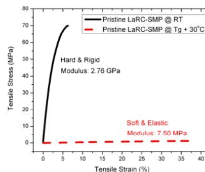
Figure 2. Mechanical properties measured at room temperature and at elevated temperature (30°C above the glass transition temperature (96°C)) of pristine LaRC shape memory polymer (LaRC-SMP)
