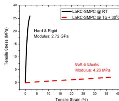
Figure 3. Mechanical properties measured at room temperature and at elevated temperature (30°C above the glass transition temperature (95°C)) of LaRC shape memory polymer composite (LaRC-SMPC).
