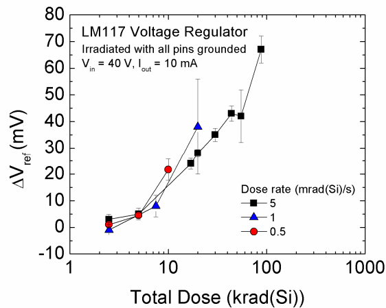
Fig. 6. Change in reference voltage vs. TID for the LM117 adjustable voltage regulator irradiated at 5, 1, and 0.5 mrad(Si)/s
