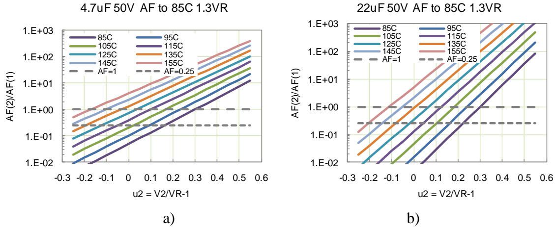
Figure 15. Variations of acceleration factors normalized to conditions V_1 = 1.3VR and T_1 = 85 °C with voltage stress factors u_2 at different temperatures T_2 from 85 °C to 155 °C for 4.7 uF 50 V capacitors (a) and 22 uF 50 V capacitors (b).
