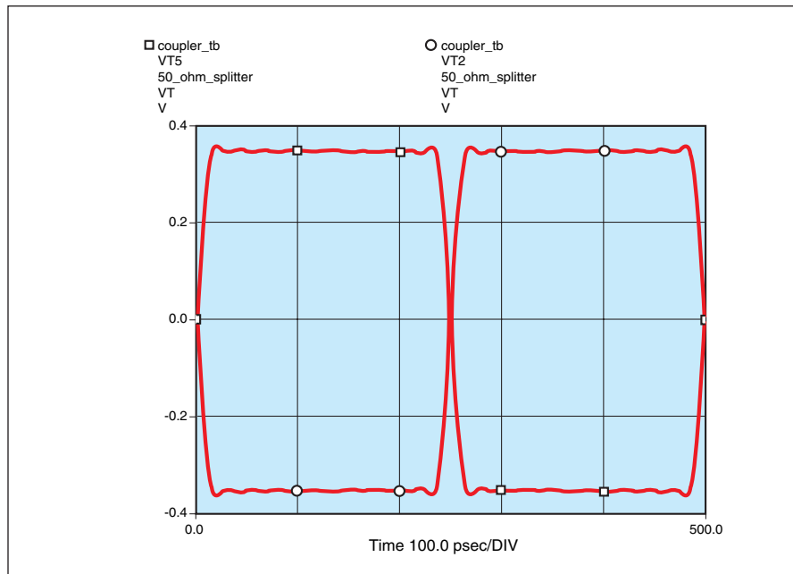
These Two Waveforms at Output Ports of a 50-Ω Power Divider are 180° out of phase with each other and resemble the input waveform.
