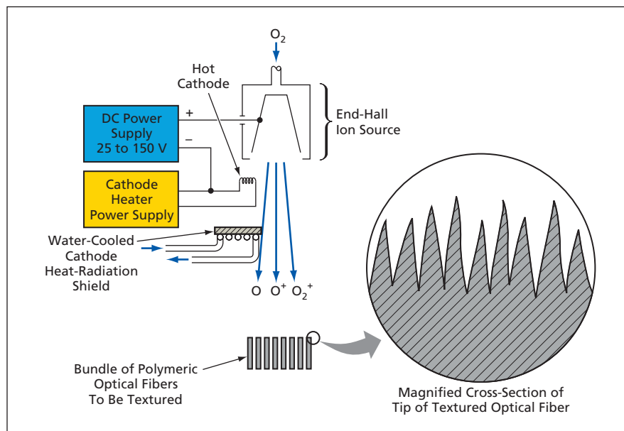
Directed Energetic Oxygen Atoms and Ions impinging on tips of polymeric optical fibers cause the tips to become textured with microscopic, approximately conical hills having large aspect ratios.
