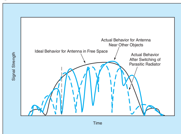
Figure 2. The Radiation Pattern Would Be Shifted and otherwise altered by switching of a parasitic radiator. At the time and position represented by the vertical dashed line, the distant terminal would be in a deep fade of the first radiation pattern but near a peak of the second (shifted) one.
