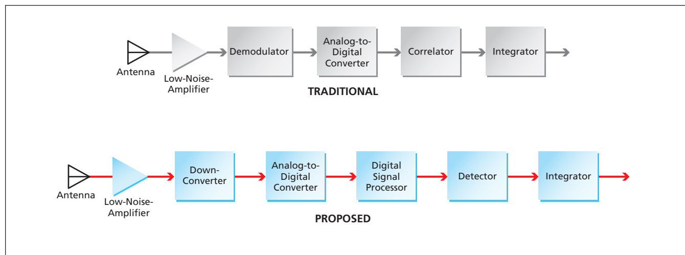
The Proposed Microwave Radiometer Receiver would include a digital signal processor that would execute interference-suppression algorithms.
