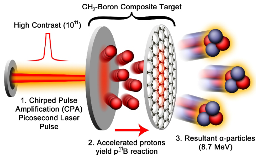
Figure 3. Composite target employing ^{11}\text{B} Boron layer impregnation in conjunction with triggering of the reaction by custom CPA laser to achieve Target Normal Sheath Acceleration (TNSA) of precursor ions. This induces a laser triggered plasma-jet from a solid target in vacuum.
