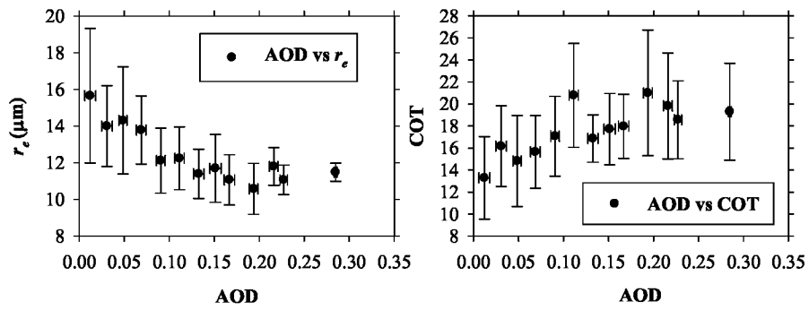
Fig. 3. On the left is the cloud droplet effective radius ( r_e ) as a function of AOD. On the right is cloud optical thickness (COT) as a function of AOD. Data are based on satellite retrievals.
