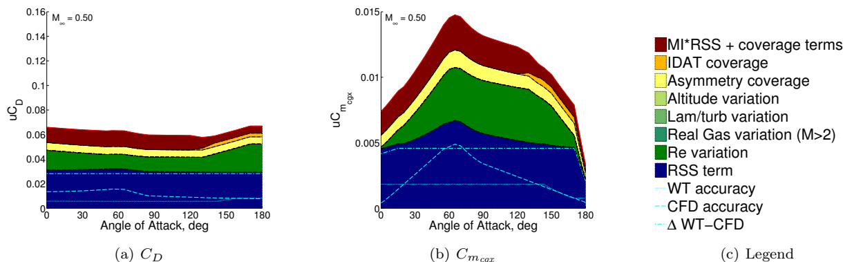
Figure 29: Uncertainty buildup, M = 0.5 .
