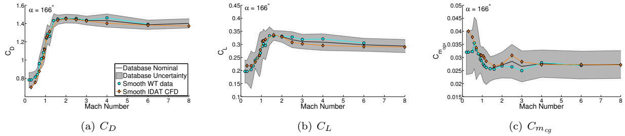
Figure 38: Nominal aerodynamic coefficients with uncertainties compared to available experimental and computational data, for \alpha = 166^\circ , M < 8
