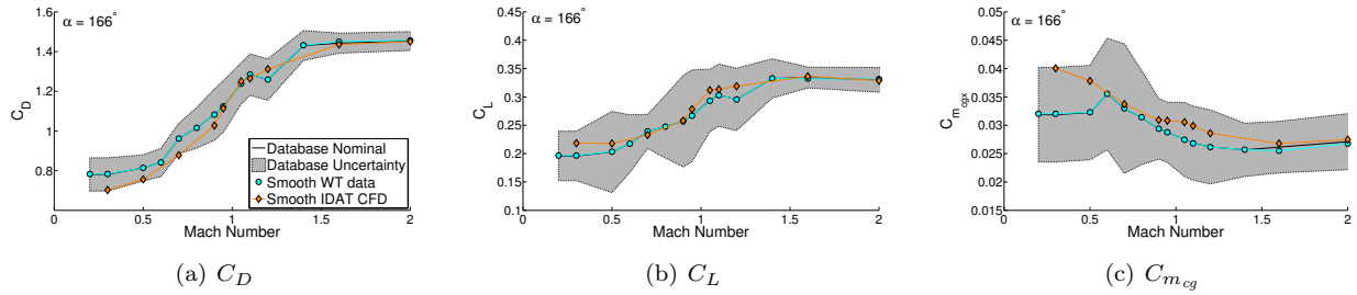
Figure 39: Nominal aerodynamic coefficients with uncertainties compared to available experimental and computational data, for \alpha = 166^\circ , M < 2 .
