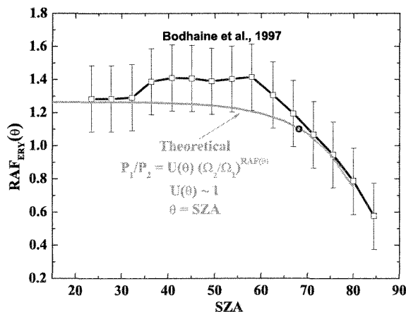
Figure 10. \text{RAF}_{\text{ERY}}(\theta) variation with \theta (SZA) for the erythemal action spectrum from data obtained at Mauna Loa Hawaii [Bodhaine et al., 1997] compared with a theoretical calculation based on equations (2) and (6) and Tables 3 and 4. The small circle is located at \theta = 68^\circ with a RAF value of 1.1.
