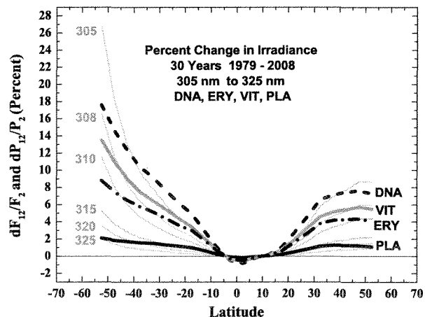
Figure 11. Percent changes dP_{12}/P_2 in DNA damage (DNA), erythemal (ERY), vitamin D (VIT), and plant growth (PLA) action spectra weighted irradiances from total change in ozone amount for 30 years (1979 to 2008). Also shown for comparison are six monochromatic dF_{12}/F_2 irradiance changes from Figure 3. The action spectra calculations are based on Tables 3 and 4 and equation (8).
