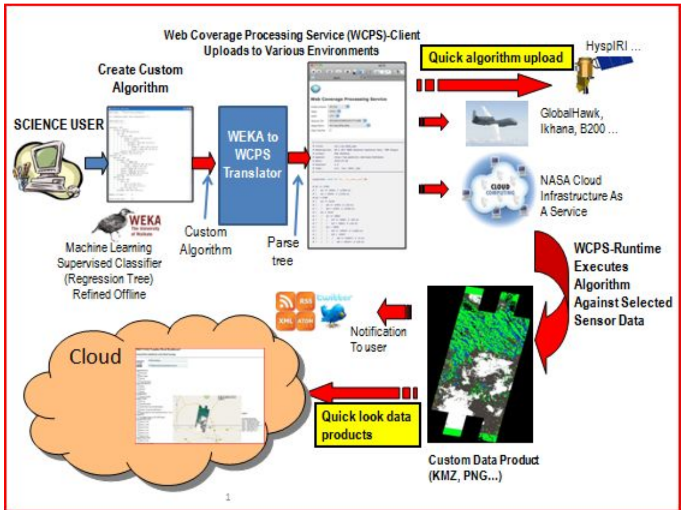
Figure 4 Top level operations concepts for WCPS in which a ground based WCPS client is used to design a algorithm and then the algorithm is uploaded to one of three environments. The user selects one of the created algorithms to run via the WCPS-R which causes the quick look data product to be produced and sent to the elastic compute cloud.
