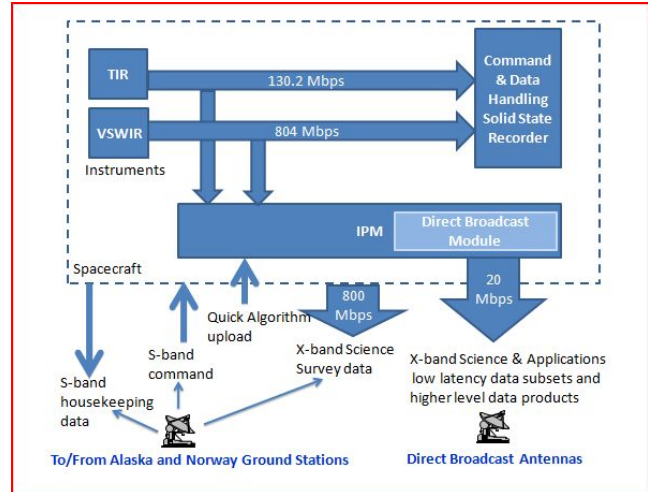
Figure3 Architecture of the IPM to be used for HypsIRI Decadal mission and possibly other NASA Decadal missions.
