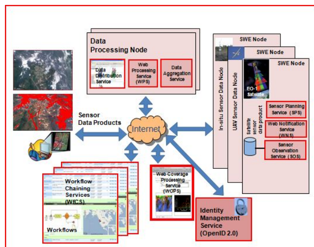
Figure 1 High level SensorWeb architecture with key components outlined in red and WCPS outlined in a heavy red line
