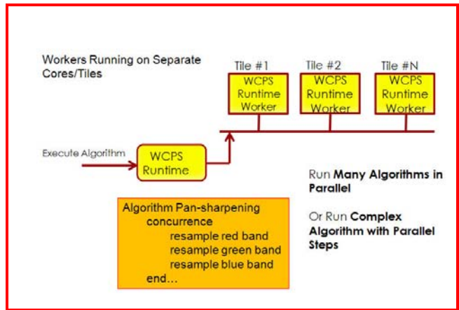
Figure 7 WCPS specified pan sharpened algorithm specified to run concurrently
