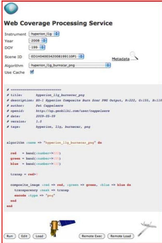
Figure 6 User interface for access to WCPS-C and WCPS-R
