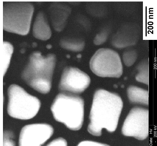
Figure 4.—a) Comparison of secondary (S) and tertiary (T) \gamma' for the six conditions of subscale LSHR.
