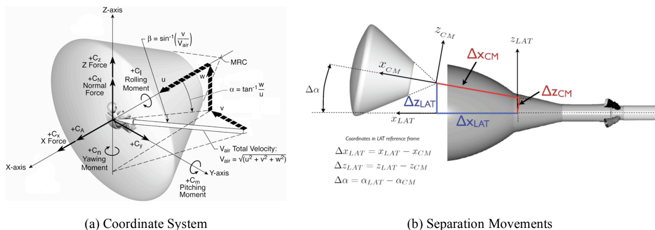
Figure 3. Coordinate System and Separation Movement Definitions.
