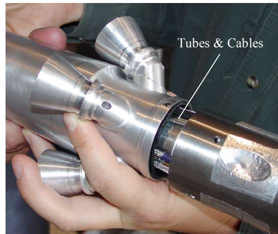
Figure 11. Routing of Instrumentation Lines Across Metric Break for Test 24-AA Model.
