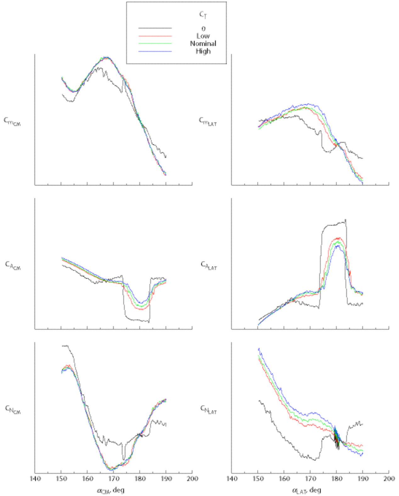
Figure 26. Effect of C_T at M_\infty = 0.50 , \beta = 0^\circ , \Delta X/D = -0.25 , \Delta Z/D = 0 , \Delta\alpha = 0^\circ .
