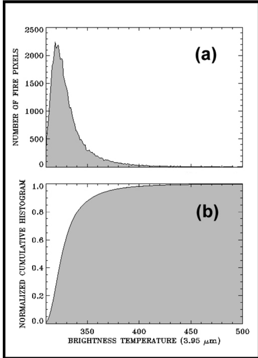
Figure 3. Fire pixels histograms compiled by Gao et al. [2007]. (a) Relative frequency plot; (b) cumulative probability plot. Note that 90% of the 4-μm temperatures were \leq 350 K.
