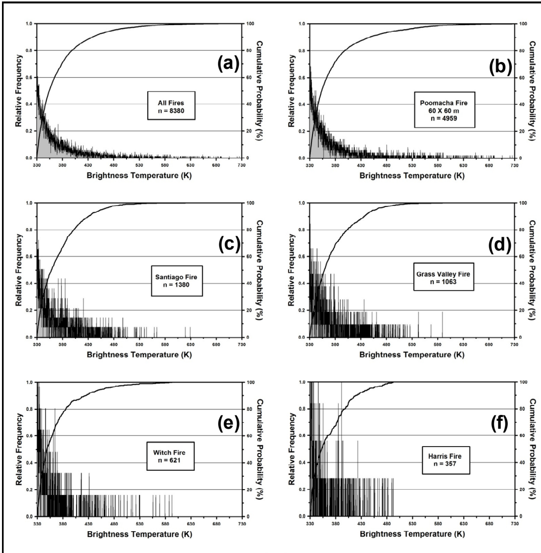
Figure 17. Relative frequency and cumulative histograms of high temperatures estimates (330 – 730 K), following aggregation of the Channel 12 (10.5 \mu\text{m} ) radiance from native resolution into 60-m HypsIRI pixels. (a) Histogram for all fires; (b) Poomacha Fire histogram, (c) Santiago Fire histogram; (d) Grass Valley Fire histogram; (e) Witch Fire histogram; and (f) Harris Fire histogram.
