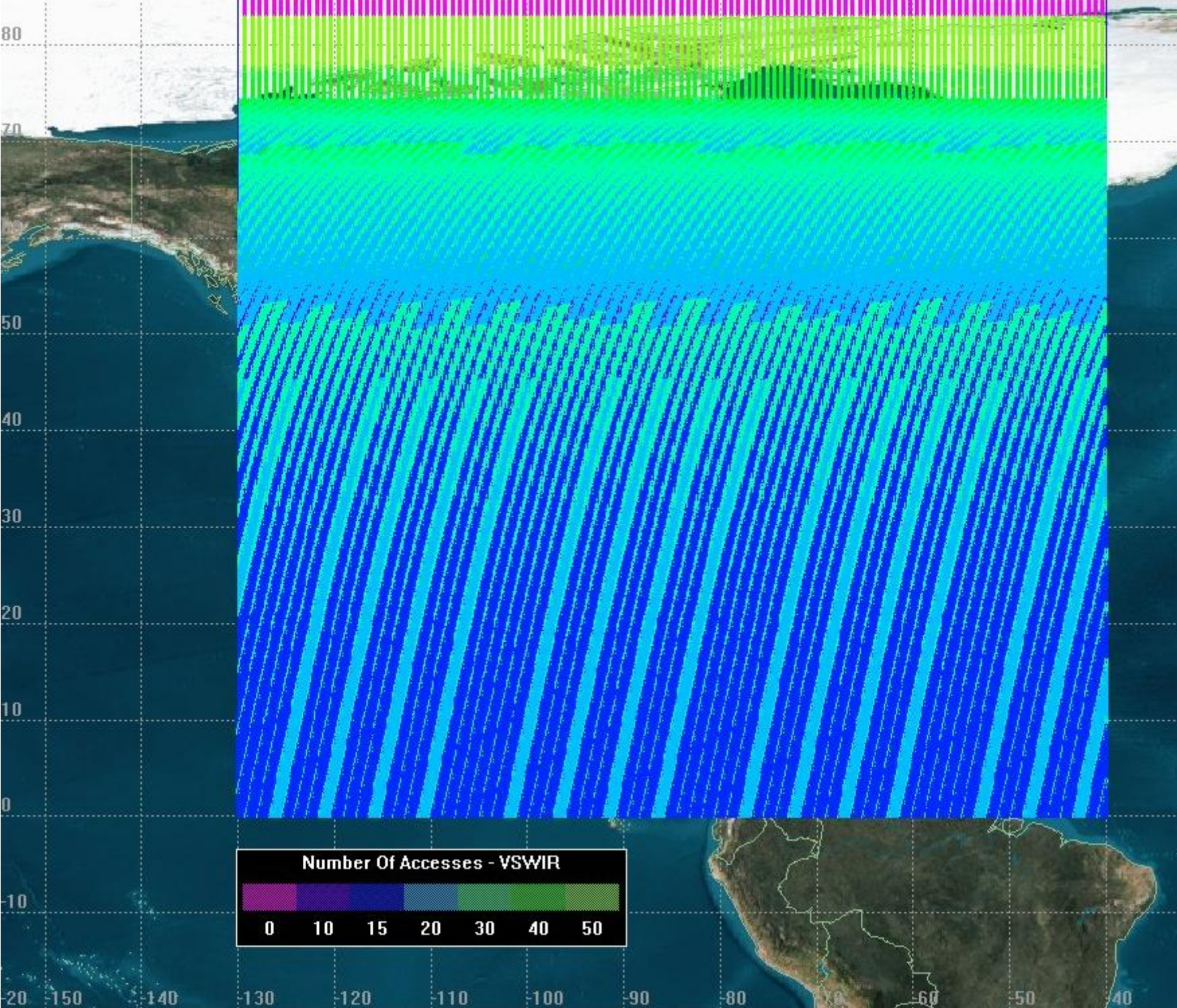
Nominal orbit: av. alt. 626.8 km, incl. 97.8°. VSWIR spectrometer FOV: 2.8° E, 10.8° W (60 m pixel GSD at nadir, 2480 cross-track pixels). R.G. Knox, NASA GSFC, Biospheric Sciences Branch, Code 614.4. Simulated with STK v9.2, August 17, 2010. Note aliasing at high latitudes.
