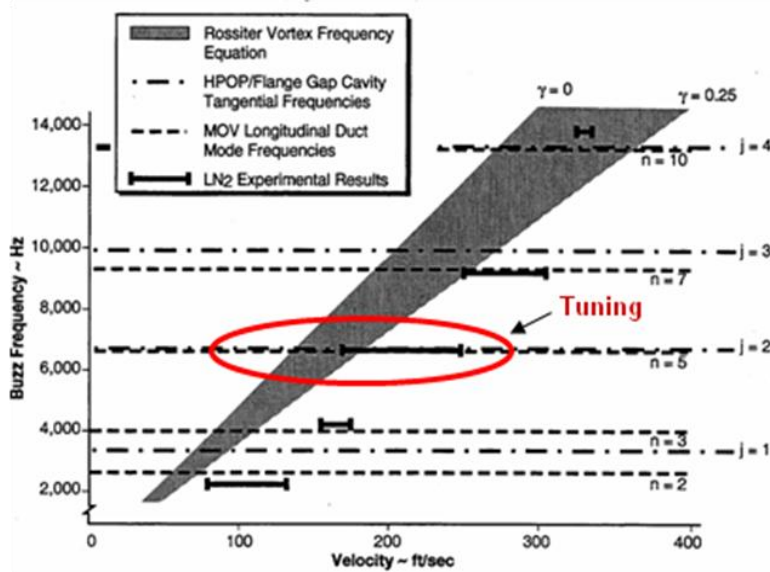
Figure 20-7. Acoustical Mechanism
