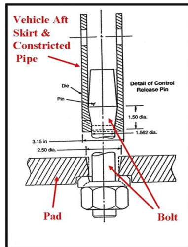
Figure 12-4. Saturn V Hold Down Post Soft Release Mechanism
