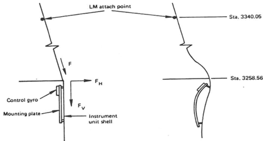
Figure 5-9. Schematic of Gyro Mounting and Local Deformation
