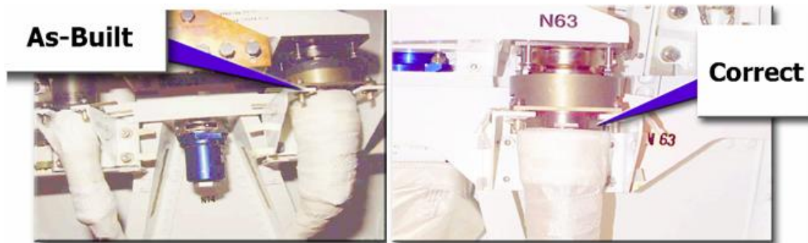
Figure 11-5. Electrical Harness as Built and Corrected
