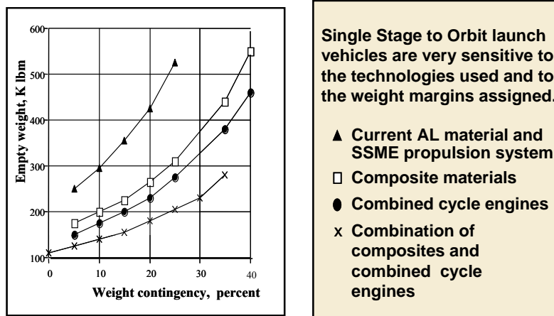
Figure 3-4. Dry Weight Versus Weight Contingency in Percent
