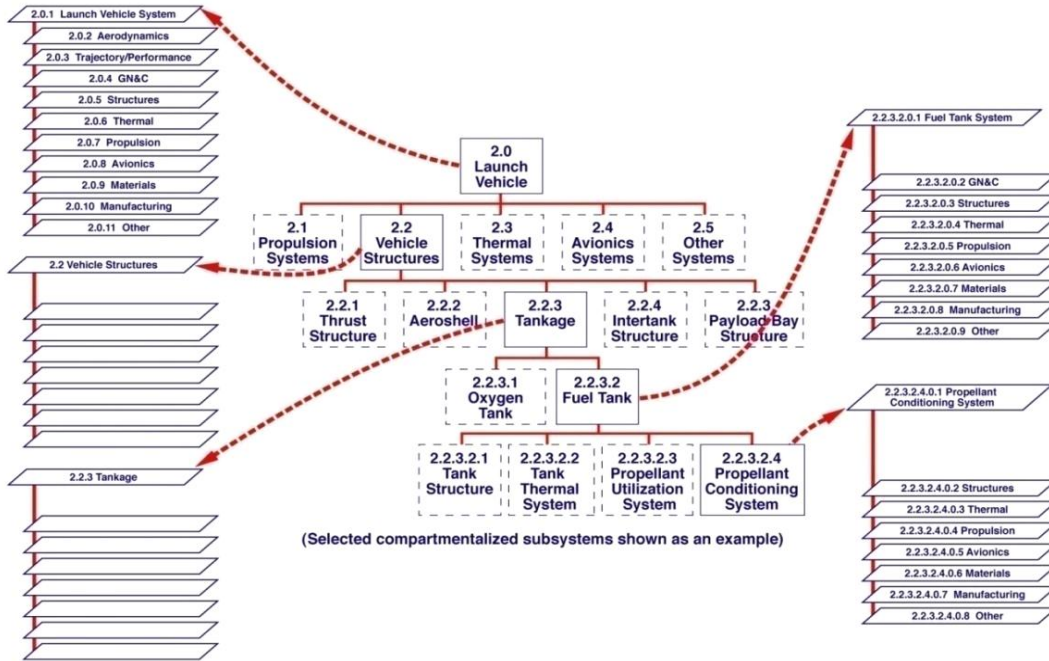
Figure 4-4. Typical Subsystems with Associated Design Functions
