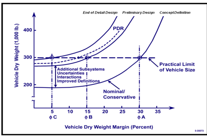
Figure 10-3. Launch Vehicle Dry weight Sensitivity to Dry Weight Margin
