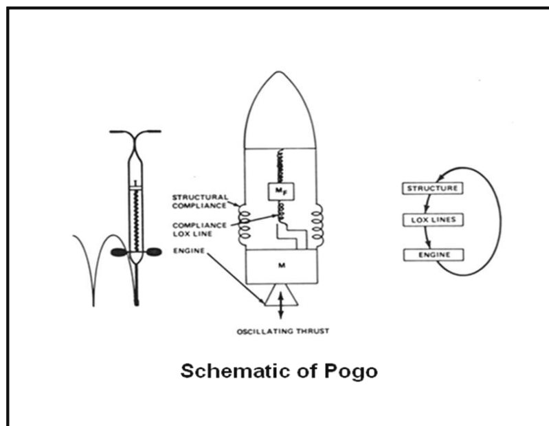
Figure 24-2. Pogo Oscillation Mechanism
