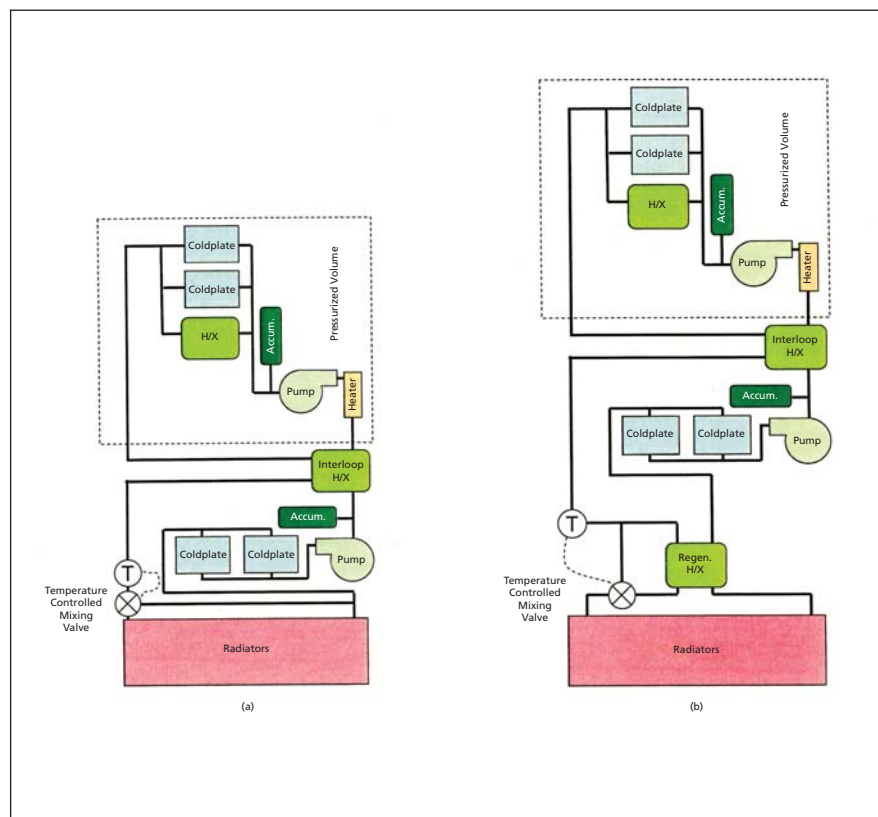
(a) Active Thermal Control System with radiator bypass; (b) Active Thermal Control System Design with regenerator bypass.
