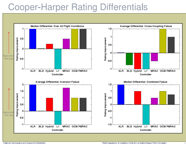
Fig. 15. Cooper-Harper Rating Improvement of Various Adaptive Control Methods
