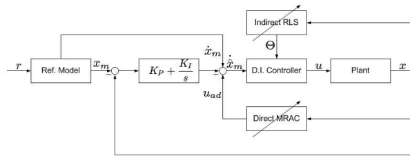
Fig. 1. Hybrid Adaptive Flight Control Architecture
