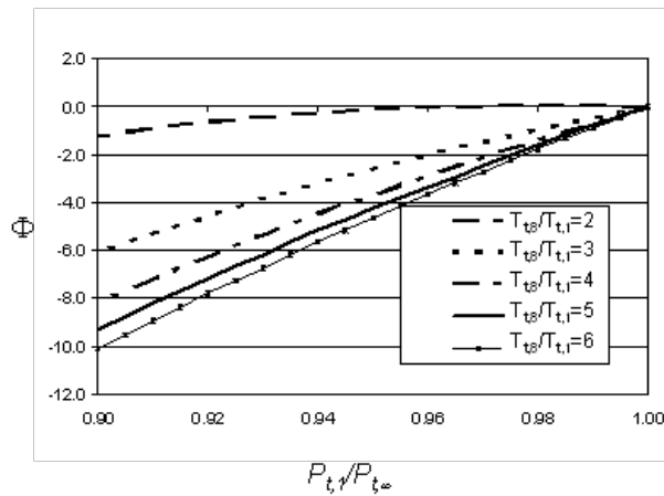
Figure 5. Amount of BLI ( P_{t,1}/P_{t,\infty} ) vs. nondimensional thrust benefit in percentage, \Phi , for turbojet-like engine without fans at various T_{t,8}/T_{t,1} . ( f = 0.029 , M_\infty = M_0 = 0.8 ).
