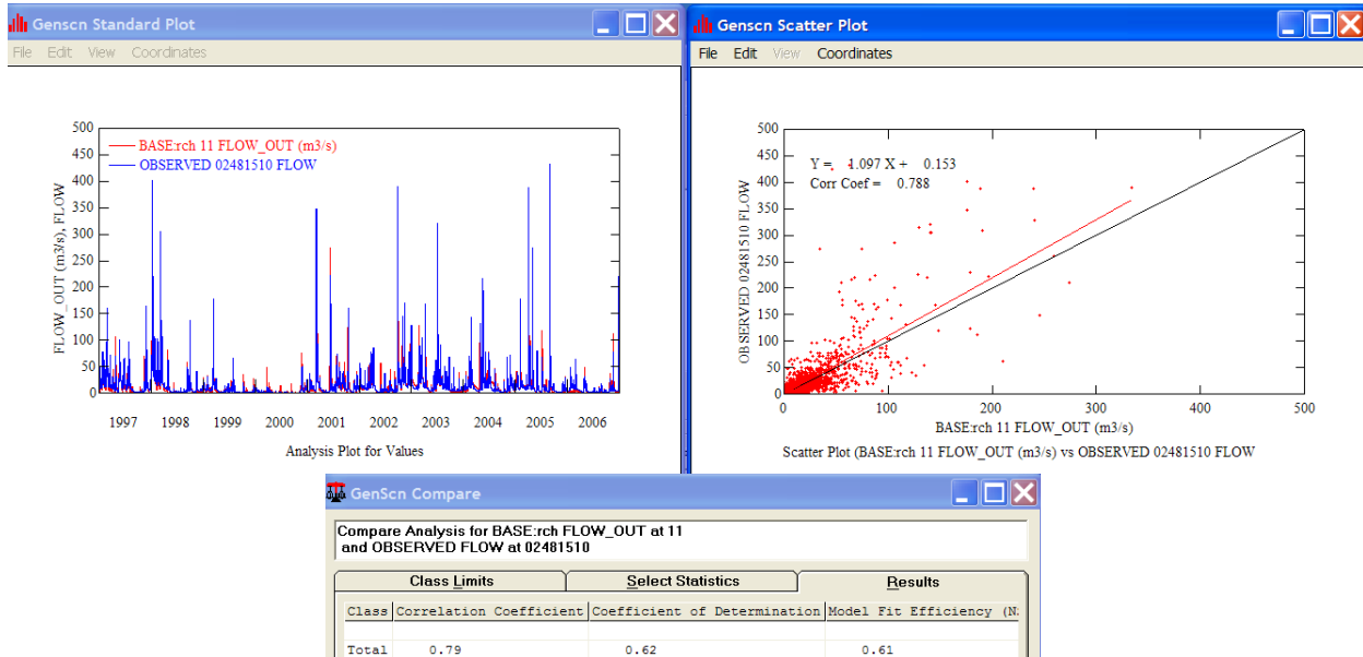
Figure 12. Calibration of the SWAT model application to Wolf River watershed.
