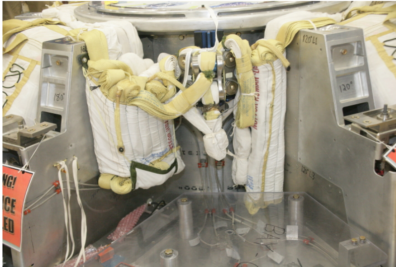
Figure 6 - Keeper Installed
