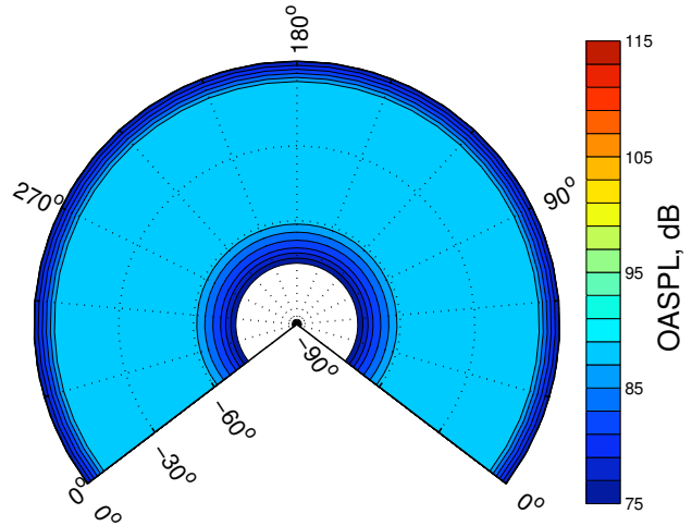
Fig. 4. Hovering flight steady loading noise OASPL hemisphere at ISA sea level conditions. ( C_T = 0.0029 , M_H = 0.66 )
