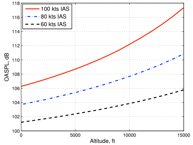
Fig. 12. Thickness noise OASPL trend for advance ratio variation to maintain constant IAS at altitude.
