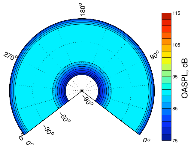
Fig. 5. Hovering flight steady loading noise OASPL hemisphere at ISA 15,000 ft altitude conditions. ( C_T = 0.0046 , M_H = 0.70 )
