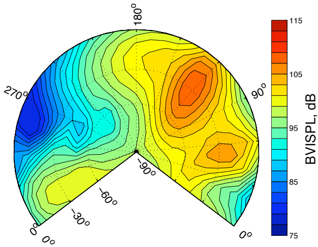
Fig. 16. 60kts IAS -6^\circ descent BVISPL hemisphere at ISA 15,000 ft conditions.
