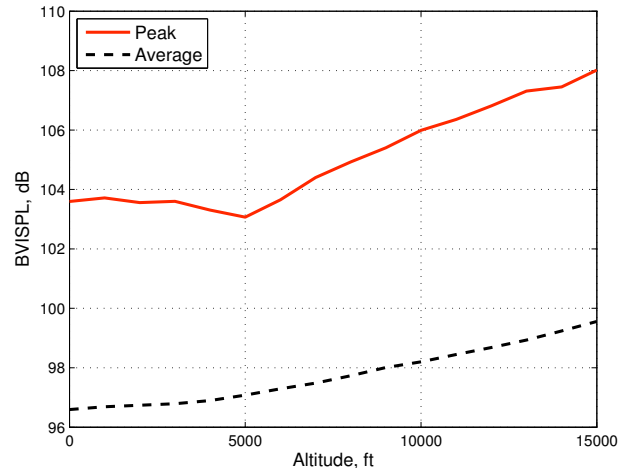
Fig. 18. Variation of BVISPL values with ISA altitude conditions for 60 kts IAS, -6^\circ descent flight.
