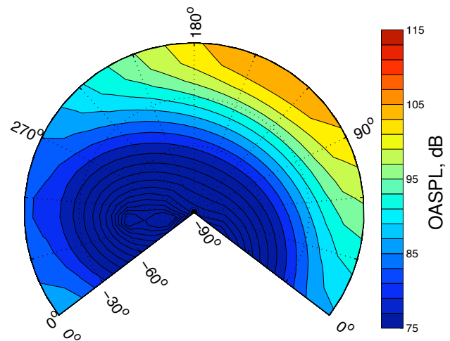
Fig. 8. 60kts IAS OASPL hemisphere of thickness noise at ISA 15,000 ft altitude conditions. ( \mu = 0.18 , M_H = 0.70 , M_{AT} = 0.89 )
