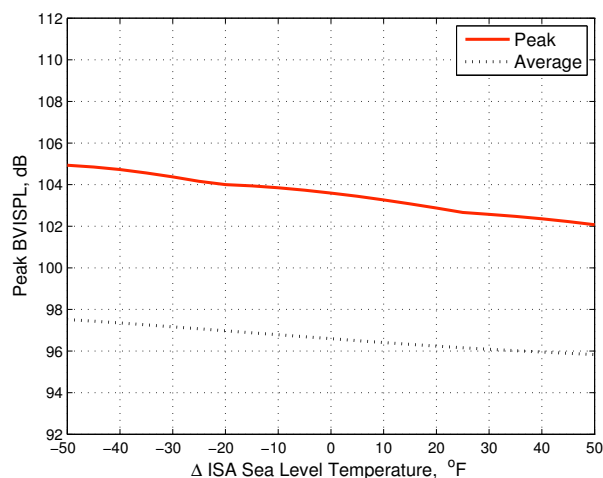
Fig. 27. Variation of BVISPL values for ISA sea level temperature variations at 60 kts IAS, -6° descent flight.
