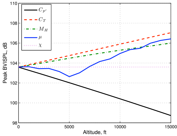
Fig. 23. Peak BVISPL trends for individual governing parameter variations with altitude.
