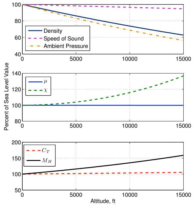
Fig. 1. (top) The variation in atmospheric and governing parameters for the ISA model. (mid/bottom) Corresponding variations in the non-dimensional governing parameters for a constant 60 kts IAS -6^\circ FPA approach.
