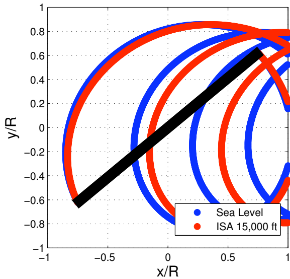
Fig. 2. “Top-view” epicycloidal wake geometry for sea level and ISA 15,000 ft advance ratios at 60 kts IAS.
