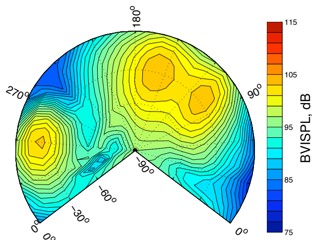
Fig. 14. 60kts IAS -6° descent BVISPL hemisphere at ISA 5,000 ft conditions.
