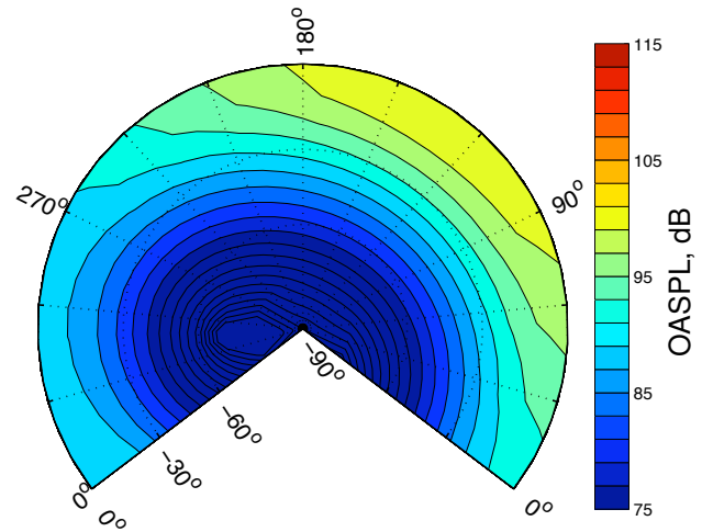
Fig. 7. 60kts IAS OASPL hemisphere of thickness noise at ISA sea level conditions. ( \mu = 0.14 , M_H = 0.66 , M_{AT} = 0.66 )
