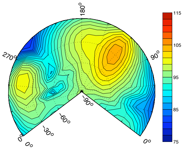
Fig. 34. 60kts TAS -6° descent BVISPL hemisphere at ISA 5,000 ft conditions. (\mu = 0.14, \chi = 0.048, C_T = 0.0034, M_H = 0.67)
