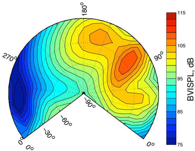
Fig. 17. 60kts IAS -6^\circ descent BVISPL hemisphere at ISA 20,000 ft conditions.
