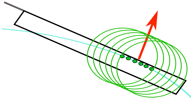
Fig. 30. Huygens' wavelet diagram of a parallel BVI, as in interaction #3 of Figure 28.
