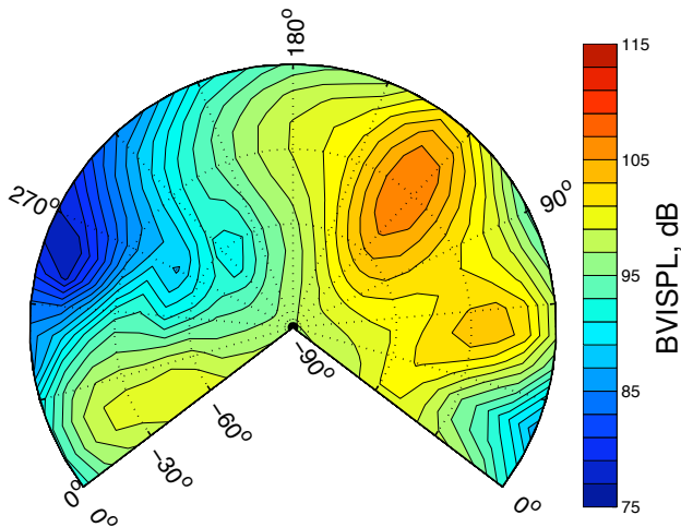
Fig. 21. 60kts IAS -6^\circ descent BVISPL hemisphere for \mu only at ISA 15,000 ft altitude conditions. (\mu = 0.18, \chi = 0.046, C_T = 0.0029, M_H = 0.66)
