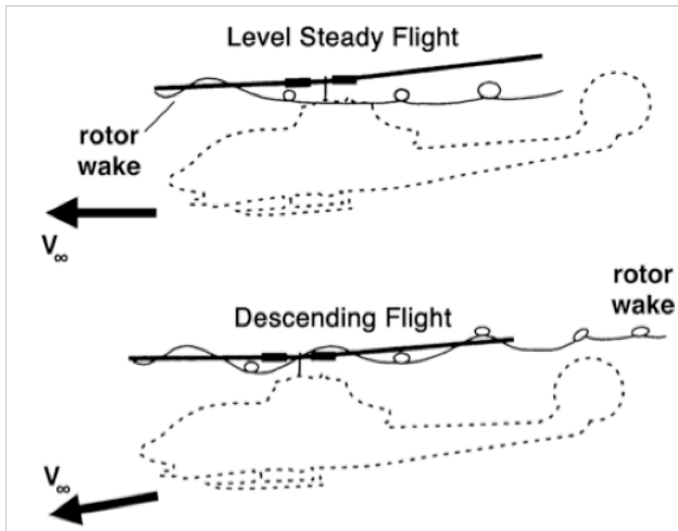
Fig. 31. The side-view geometry of the wake is set by the rotor inflow and determines the “miss-distance” between the vortices and blades during BVI. From Reference 25.
