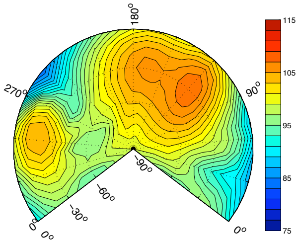
Fig. 20. 60kts IAS -6^\circ descent BVISPL hemisphere for C_T only at ISA 15,000 ft altitude conditions. (\mu = 0.14, \chi = 0.046, C_T = 0.0046, M_H = 0.66)
