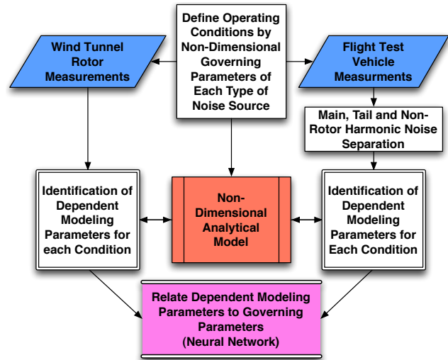
Fig. 3. A flowchart describing the FRAME method for developing rotorcraft source noise models.
