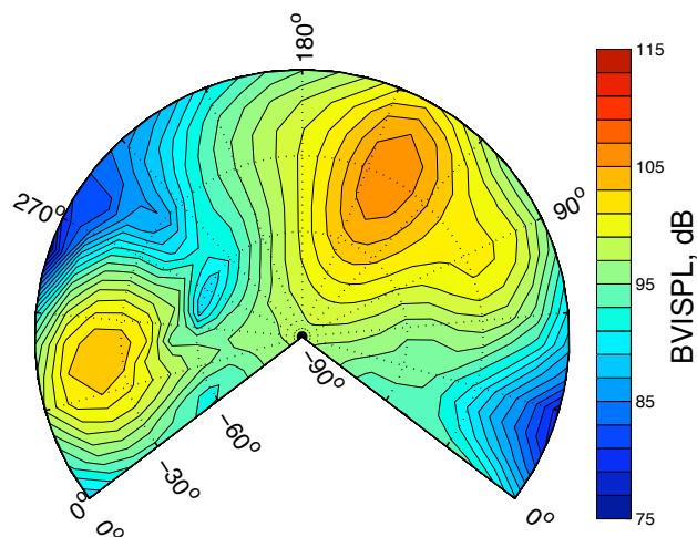
Fig. 15. 60kts IAS -6° descent BVISPL hemisphere at ISA 10,000 ft conditions.
