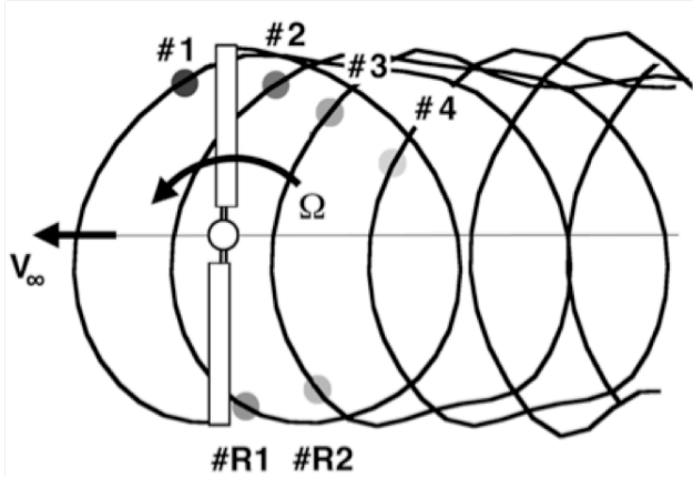
Fig. 28. The top-view geometry of the wake is set by the rotor advance ratio and hover tip Mach number and determines the BVI locations and interaction angles. From Reference 25.
