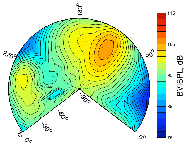
Fig. 26. 60kts IAS -6° descent BVISPL hemisphere at ISA sea level -50 °F conditions.
