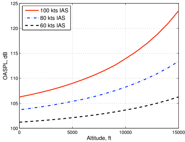
Fig. 9. Peak OASPL thickness noise level variation for ISA altitude conditions for constant IAS flight.
