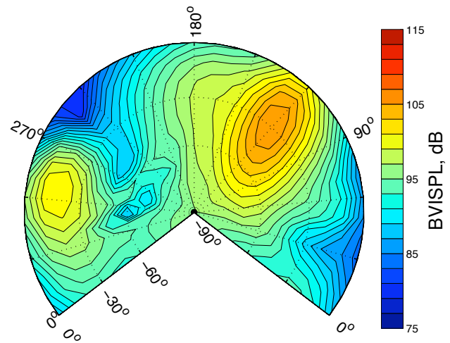
Fig. 36. 60kts TAS -6° descent BVISPL hemisphere at ISA 15,000 ft conditions. (\mu = 0.14, \chi = 0.064, C_T = 0.0046, M_H = 0.70)
