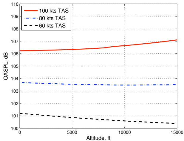
Fig. 38. Peak OASPL thickness noise level variation for ISA altitude conditions for constant TAS flight.
