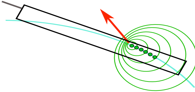
Fig. 28. The top-view geometry of the wake is set by the rotor advance ratio and hover tip Mach number and determines the BVI locations and interaction angles. From Reference 25.
