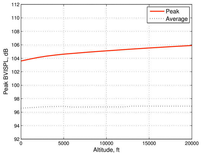
Fig. 37. Variation of BVISPL values for ISA altitude conditions at 60 kts TAS, -6° descent flight.
