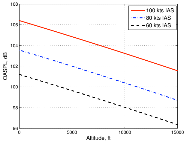
Fig. 10. OASPL variation in thickness noise for ambient pressure variation per ISA altitude conditions.
