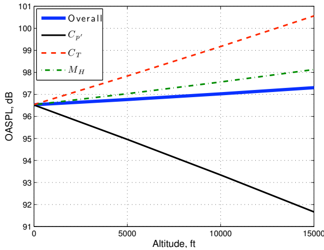
Fig. 6. (a) Variation in steady loading noise OASPL (blue) with ISA altitude conditions. (b) OASPL variations associated with individual governing parameter variations with ISA altitude conditions.
