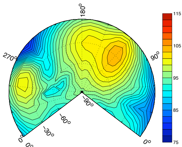
Fig. 13. 60kts IAS -6° descent BVISPL hemisphere at ISA sea level conditions.
