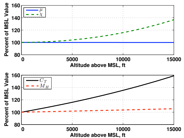
Fig. 32. The relative variation in non-dimensional governing parameters with ISA altitude for a Bell 206B3 in 60 kts TAS -6.0^\circ descending flight.
