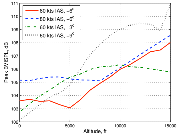
Fig. 24. Peak BVISPL trend for varying ISA altitude conditions at different dimensionally-defined flight conditions.
