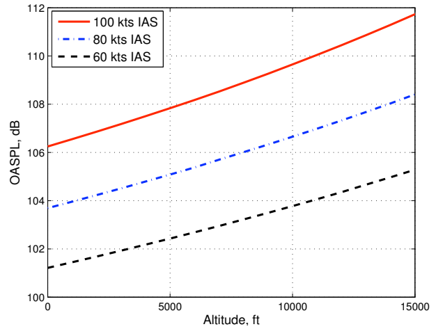
Fig. 11. Thickness noise OASPL trend for hover tip Mach number variation with temperature at altitude.
