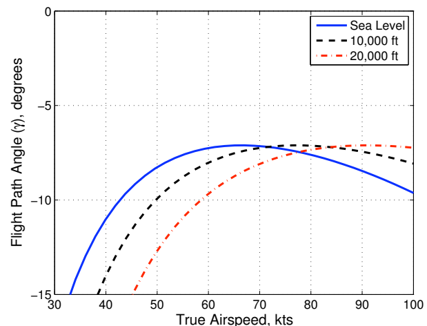
Fig. 33. A plot of the dimensionally-defined zero wake skew ratio flight conditions at various altitudes.
