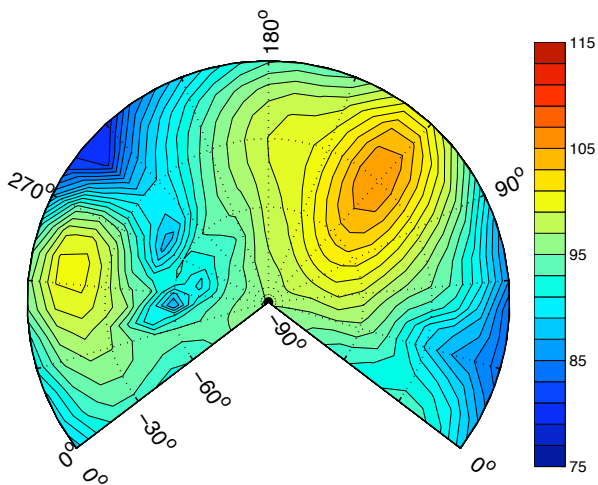
Fig. 35. 60kts TAS -6° descent BVISPL hemisphere at ISA 10,000 ft conditions. (\mu = 0.14, \chi = 0.054, C_T = 0.0039, M_H = 0.68)
