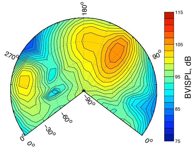
Fig. 22. 60kts IAS -6^\circ descent BVISPL hemisphere for M_H only at ISA 15,000 ft altitude conditions. (\mu = 0.14, \chi = 0.046, C_T = 0.0029, M_H = 0.71)
