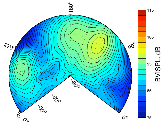
Fig. 19. BVISPL hemisphere at 15,000 ft ISA altitude ambient pressure with \mu , \chi , C_T and M_H held at ISA sea level values.
