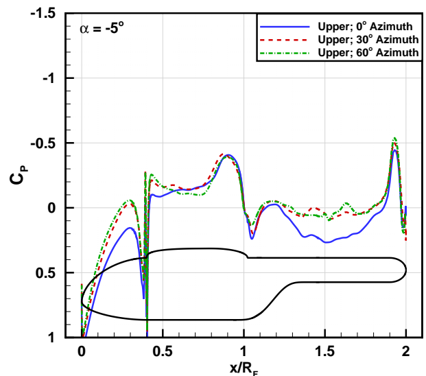
Fig. 30. Upper fuselage centerline C_p values for the baseline rotor/fuselage simulation at \alpha = -5^\circ for varying rotor azimuth angles.
