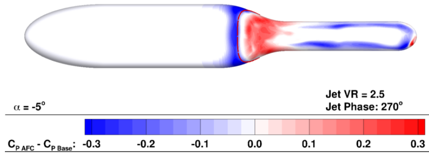
Fig. 20. Bottom view of the computed C_p difference between the baseline and AFC isolated fuselage at \alpha = -5^\circ case.
