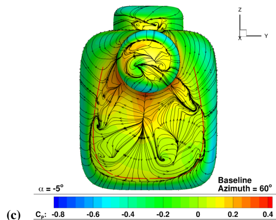
Fig. 26. Rear ramp view of the baseline rotor/fuselage simulation for the \alpha = -5^\circ case. Surface C_p contours with surface restricted streamlines at (a) \psi = 0^\circ , (b) \psi = 30^\circ , and (c) \psi = 60^\circ . (Simulation parameters: \mu = 0.35 , CT/\sigma = 0.08 , M_\infty = 0.2093 )
