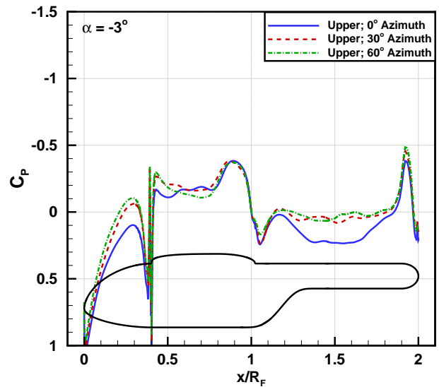
Fig. 28. Upper fuselage centerline C_p values for the baseline rotor/fuselage simulation at \alpha = -3^\circ for varying rotor azimuth angles.
