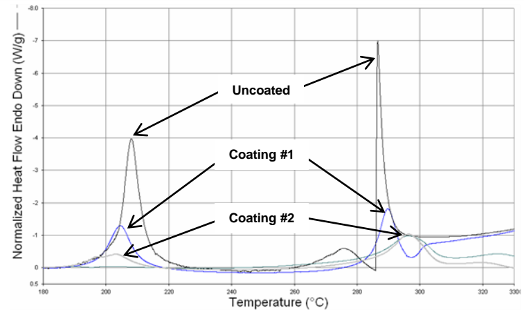
Preliminary results show reduced heat flow in exotherms of coated Toda 9100 NMC cathode. Data was collected at PSI.
