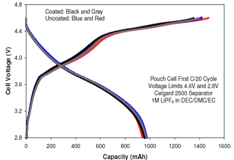
Cells containing uncoated and coated TODA 9100 NMC (2 cells of each) display similar first cycle capacity. Data was collected at PSI.
