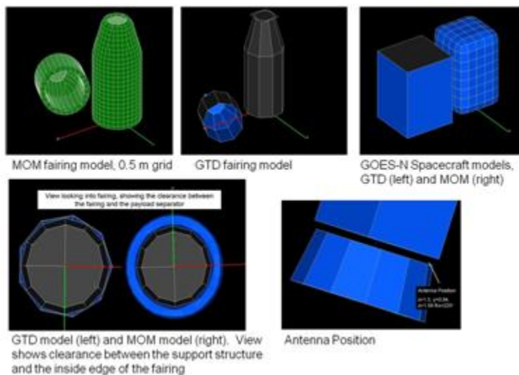
Figure 7: MOM and UTD (GTD) Models of Fairing, Spacecraft, Separation Plane, and Antenna
