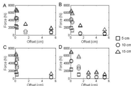
Experimental suit impact force data vs. offset. Three different drop heights (5 cm, 10 cm and 15 cm) and four different EVA suit analog pressurizations were used: A. 27 kPa; B. 29 kPa; C. 32 kPa; D. 33 kPa. Three trials were performed at each test condition.
