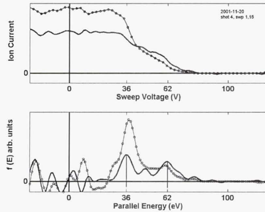
Figure 22: Upper panel: collimated RPA I-V characteristic for first (heavy line) and last (circles) sweeps of a 15-sweep set spanning the time interval from 0.4 seconds into the discharge to 0.8 seconds.
