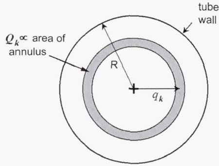
Figure 10: The transmission function for a given radius q_k is weighted by the ratio Q_k of the annular area to the tube cross-sectional area \pi R^2 .
