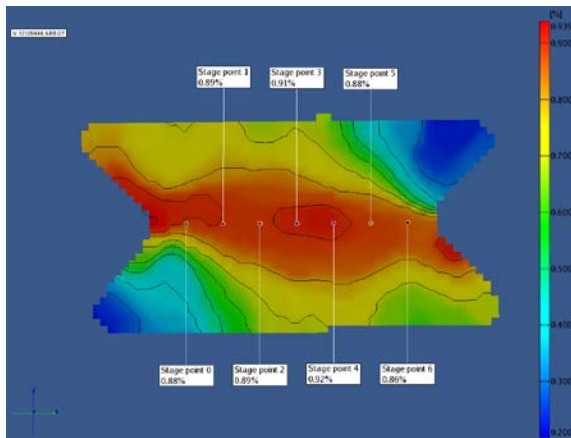
Figure 10. Sample ABB-7: 3D Major Strain Field at Break and Major Strain vs Time at Stage Points 0-6.
