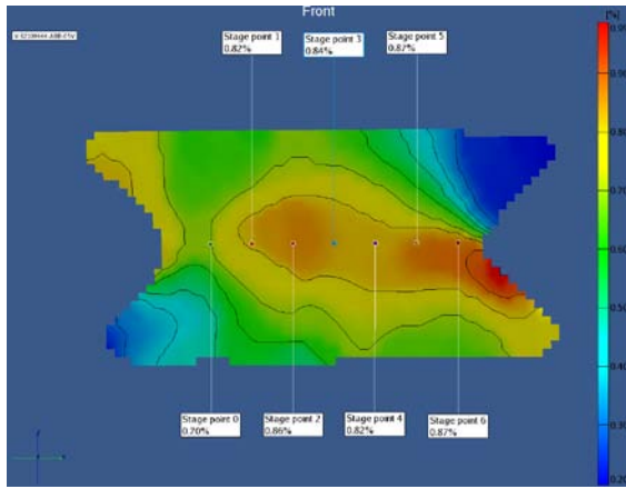
Figure 9. Sample ABB-05: 3D Major Strain Field at Break and Major Strain vs Time at Stage Points 0-6.
