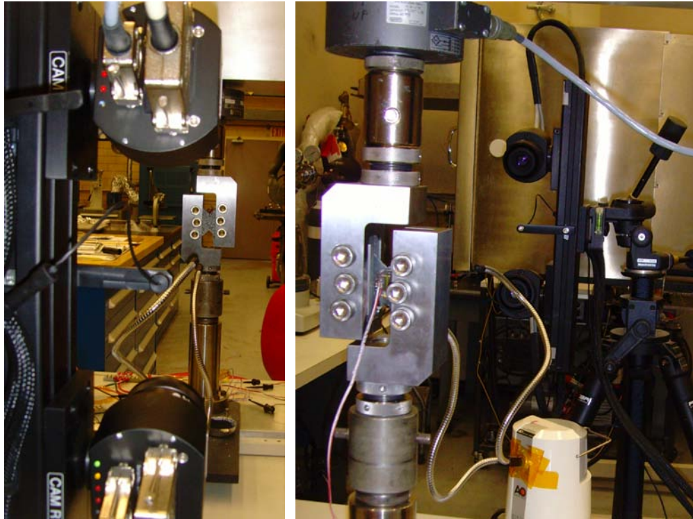
Figure 5. Dual Camera Position Showing Vertical Alignment (front and back views)
