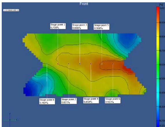
Figure 11. Sample ABB-10: 3D Major Strain Field at Break and Major Strain vs Time at Stage Points 0-6.
