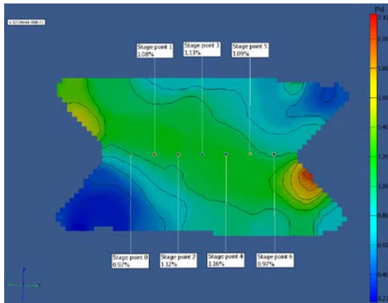
Figure 6. Sample ABB-01: 3D Major Strain Field at Break and Major Strain vs Time at Stage Points 0-6.
