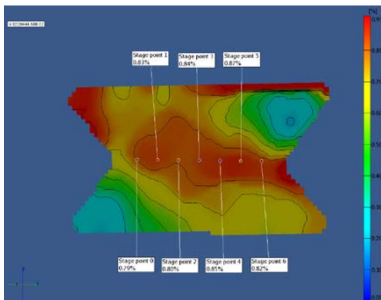
Figure 7. Sample ABB-02: 3D Major Strain Field at Break and Major Strain vs Time at Stage Points 0-6.
