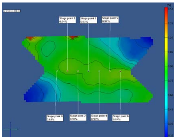
Figure 8. Sample ABB-04: 3D Major Strain Field at Break and Major Strain vs Time at Stage Points 0-6.
