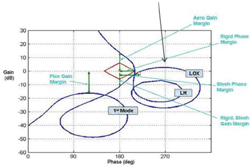
Figure 13. Notional depiction of Ares-I FCS gain and phase margins (upper-stage example).
