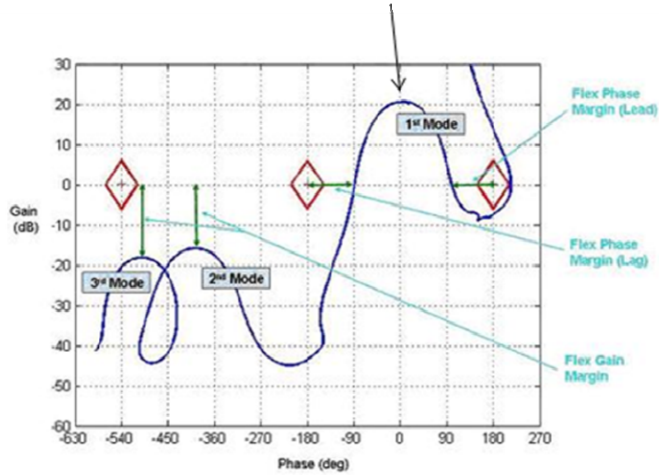
Figure 12. Notional depiction of Ares-I FCS gain and phase margins (first-stage example).
