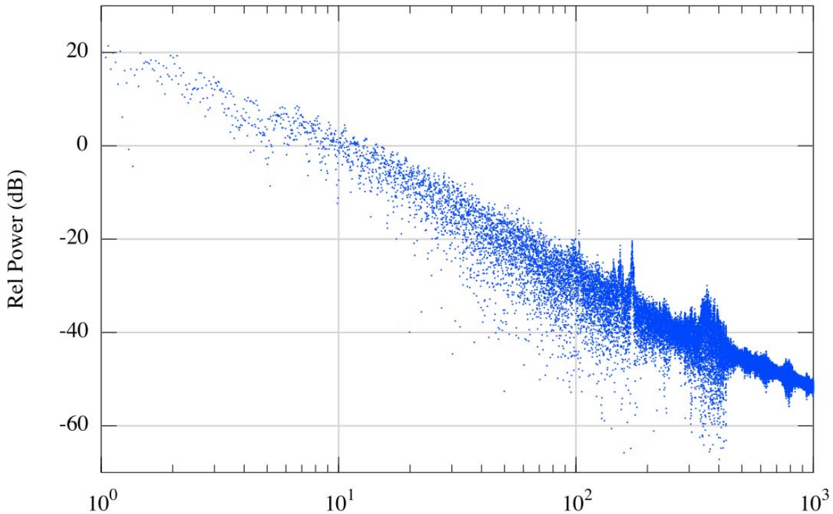
Figure 9. Low pass filtered X-axis CG#1 accelerometer data from CM water drop test.
