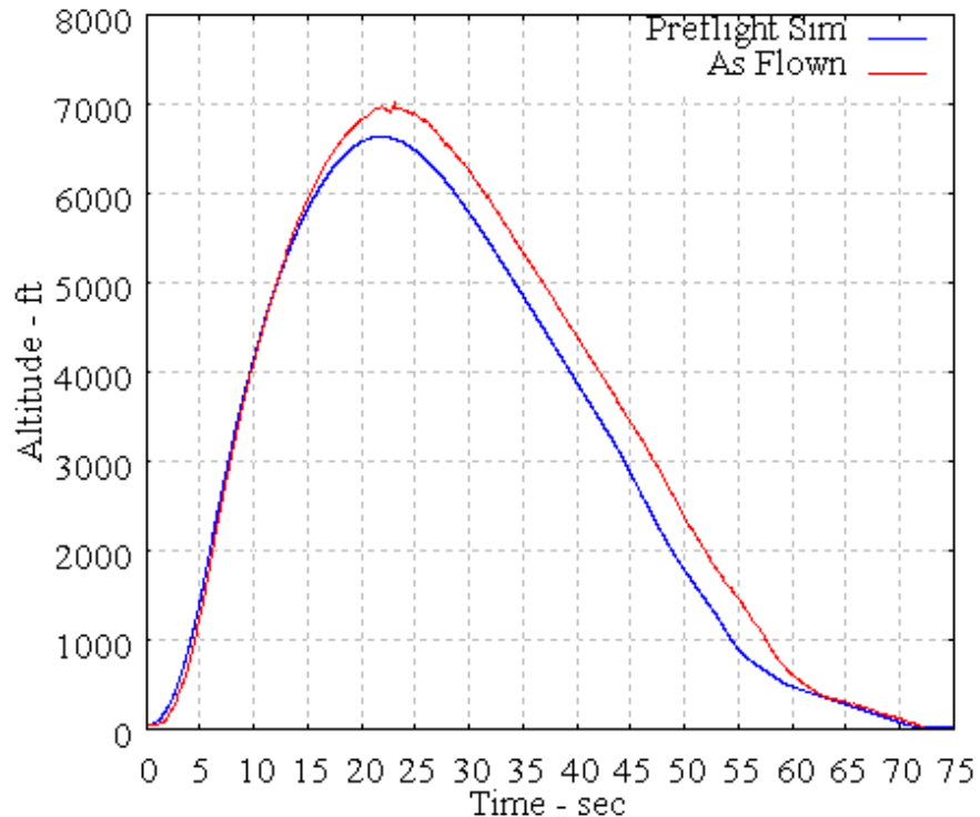
Figure 4. CM altitude versus time.
