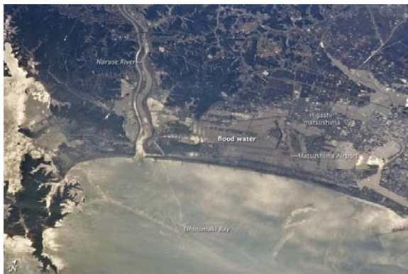
Figure 5 Northern coast of Japan from the International Space Station two days after the devastating tsunami. Image courtesy NASA.
