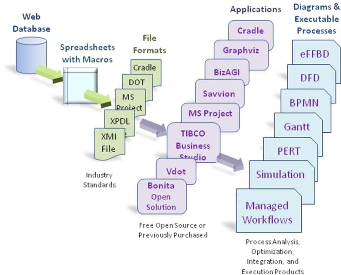
Figure 2. Process Engineering Tool Suite
