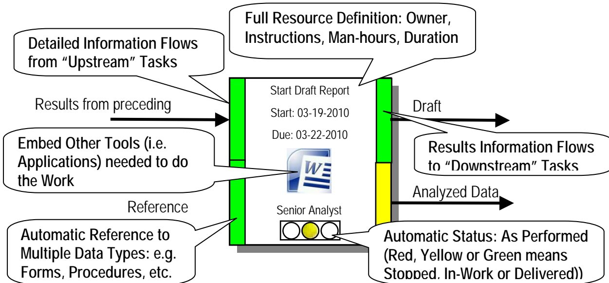
Figure 6. Vdot Smart Task
