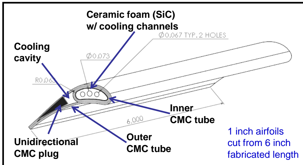
Internally Cooled Vane
