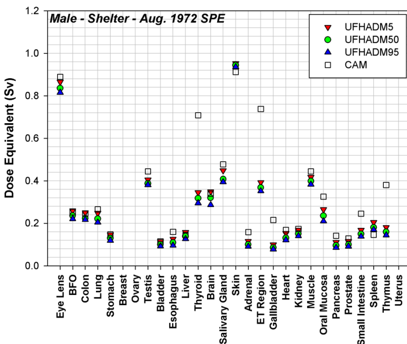
Figure 3. Organ dose equivalents for Earth-based male phantoms (August 1972 SPE, 10 \text{ g cm}^{-2} aluminum equivalent shielding) (1)
