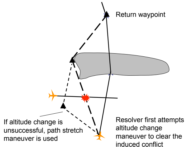
Fig. 10 Resolution of weather avoidance induced conflict.
