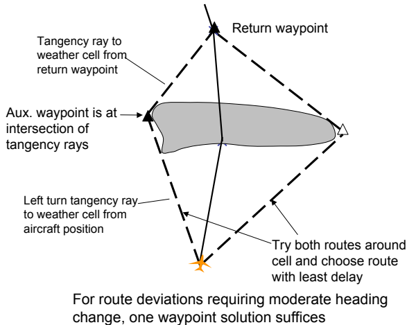
Fig. 9 Basic weather cell avoidance algorithm.
