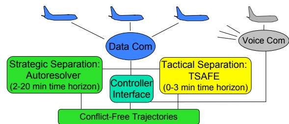
Fig. 1 Architecture of Advanced Airspace Concept.
