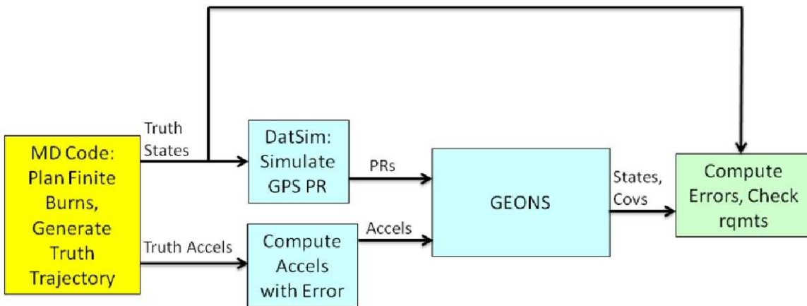
Figure 2. Simulation Methodology.
