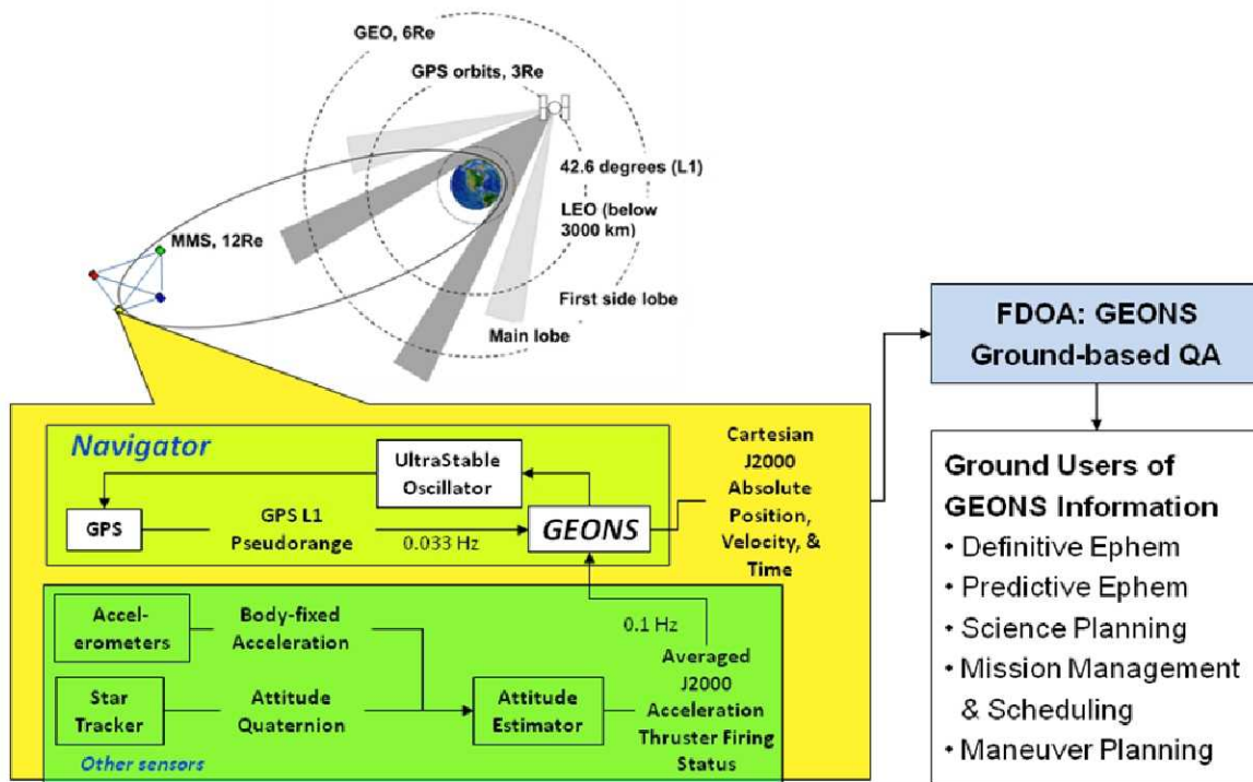
Figure 1. Navigation Concept and Onboard Configuration.
