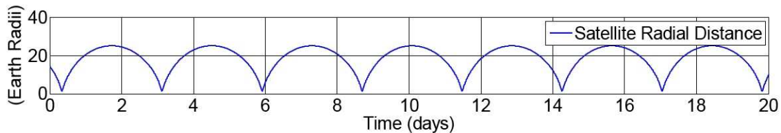
Figure 4. Satellite Orbital Radius in Earth Radii for Phase 2b.
