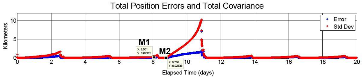
Figure 17. Baseline RSS Position Error and Covariance.
