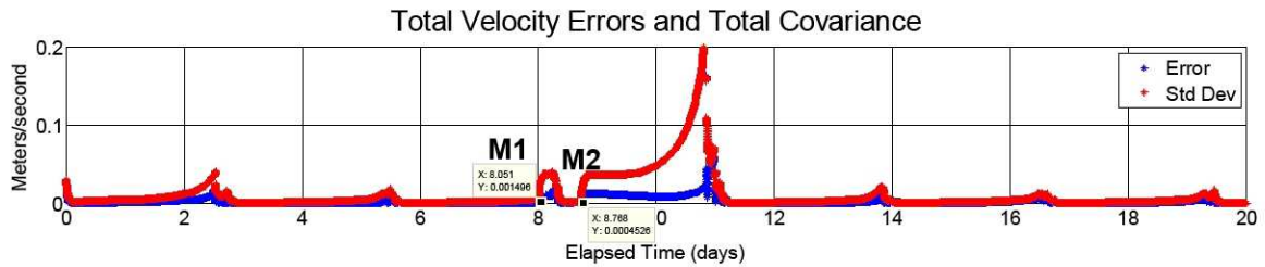
Figure 18. Baseline RSS Velocity Error and Covariance.
