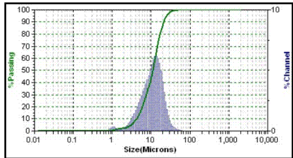
Figure 2d. Microtrac results for <20 μm sieve fraction.
