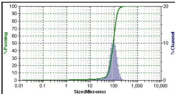
Figure 2a. Microtrac results for 75- 90 μm sieve fraction.
