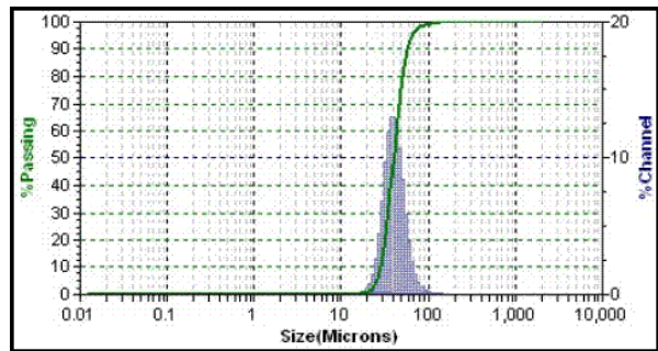
Figure 2c. Microtrac results for 20-45 μm sieve fraction.
