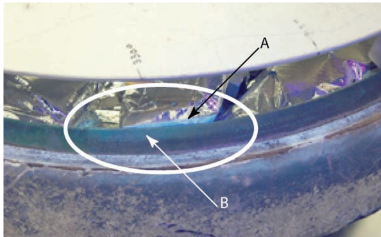
Figure 21. Black light photograph of MLI blankets (a) Outgassing from MLI and (b) also appears on the outer edge of the sealing ring.
