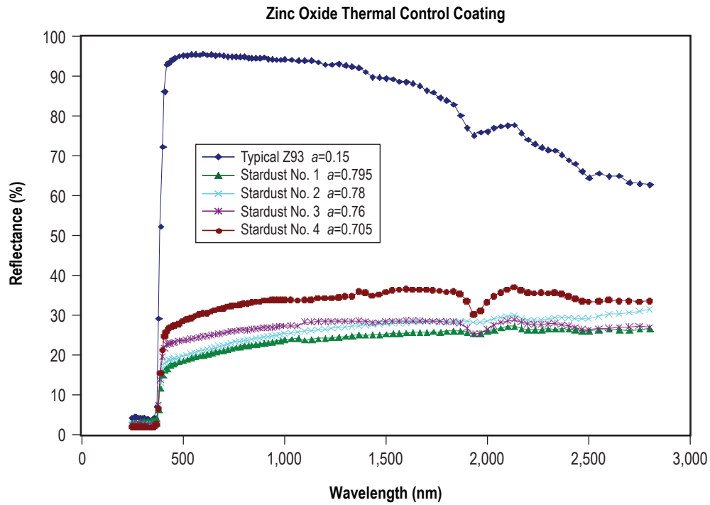
Figure 10. Z93 reflectance comparison.
