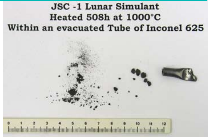
This illustrates the condition of Inconel tubes and powder following reaction at 1000 °C (1832 °F) for 500 hours. Note the “clinkering” of the powder.
