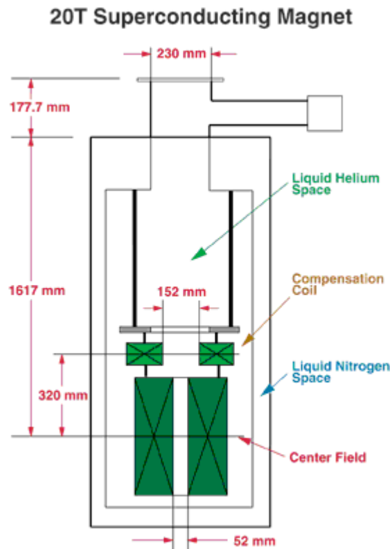
Figure 6 Schematic of the 20 T Superconducting magnet
