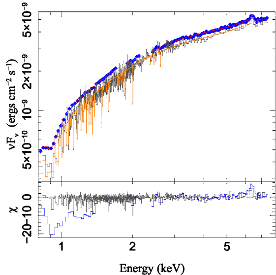
FIG. 5.— Suzaku (blue diamonds) and Chandra -HETG (grey histogram; \pm 1^{\text{st}} order HEG only) data from observation 4. The model consists of absorbed disk and powerlaw components, broad and narrow gaussian lines in the Fe K \alpha region, and absorption lines from a variety of highly ionized species, including from Fe xxv at \approx 6.7 keV. Additionally, we modify the HETG spectra by dust scattering and a pileup term (see text). The Suzaku and HETG spectra have not been renormalized with respect to one another. The residuals shown here are for this joint model fit with all broad and narrow line normalizations (both emission and absorption) set to zero.
