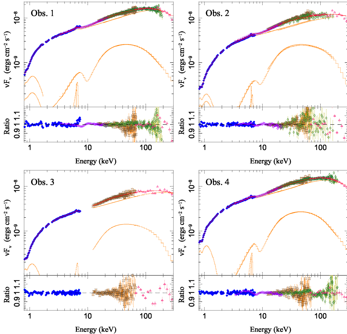
FIG. 11.— Same as Fig. 10, but for the non-thermal corona, low kT_{\text{seed}} ecpair model fits. The following model components are shown: the summed model with the reflection component excluded, the reflection component by itself, the broad and narrow Fe K\alpha line components, the seed photons without Comptonization applied, and the additional disk component with peak temperature tied to the seed photon peak temperature. Neutral and ionized absorption are applied to all shown model components.
