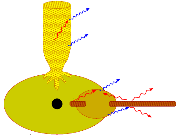
FIG. 9.— Possible X-ray emission geometry of the Cyg X-1 system. Part of the soft X-rays likely come from an accretion disk, which may be truncated at its inner edge by a hot corona. Two possible (of many suggested) geometries are shown for this corona: a torus, and a quasi-spherical cloud. In some models, the disk can reform in the inner regions of the accretion flow (Mayer & Pringle 2007). The corona will Compton upscatter a fraction of the disk component(s) soft X-rays to hard X-rays. Whether or not the corona envelops the disk(s) determines whether or not an additional, unComptonized disk component should be present in the spectra. (If the disk reforms on the inner edge of a toroidal corona, for example, a fraction of its soft X-rays will not intersect the corona.) Hard X-rays will be reprocessed into reflection/fluorescent line components, predominantly by the outer disk. Finally, the jet might contribute to the observed X-ray emission via synchrotron and synchrotron self-Compton emission.
