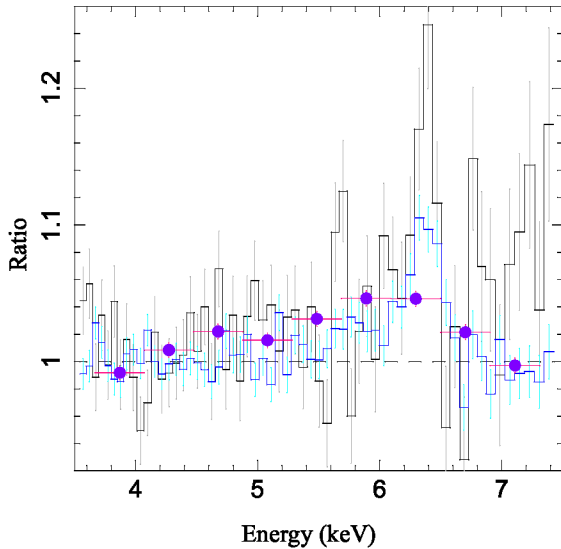
FIG. 8.— Suzaku (blue line), Chandra -HEG (grey line), and RXTE -PCA (purple diamonds) residuals from fitting an absorbed powerlaw to the 3.5–4.5 keV and 7–7.5 keV regions simultaneously. The Chandra -HEG data have been binned to match approximately the binning of the Suzaku data.
