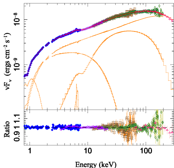
FIG. 12.— Same as Fig. 10, but only showing observation 4 for the multiple eqpair component fit (see text). The following model components are shown: the two individual eqpair components with their reflection components excluded, the reflection component of the dominant eqpair spectrum, the broad and narrow Fe K\alpha line components, and the unscattered disk component.
