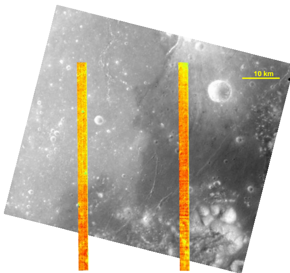
Figure 1. Diviner CF data swaths (cycle 10) over Apollo 15 metric mapping camera (frame 972) image of the dark Taurus Littrow LPD and adjacent lighter mare. Diviner data colors correspond to CF values from approximately 8.3 (yellow) to 8.4 (red).
