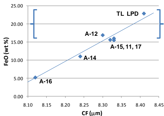
Figure 2. Correlation of Diviner CF values with sample FeO concentrations for the six Apollo sites plus the Taurus Littrow LPD. Brackets denote the range of pyroclastic glass bead compositions [3].
