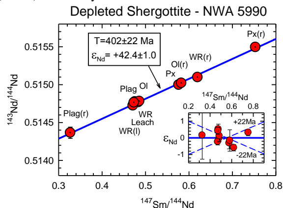
Figure 1. Sm-Nd isochron of NWA 5990.
