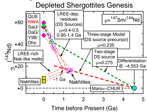
Figure 4. \epsilon_{\text{Nd}} vs. T(age) of dep. sherg. & nakhlites.
