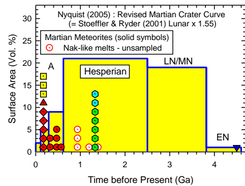
Figure 5. Age distributions of Martian Rocks.
