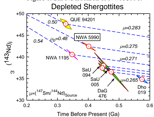
Figure 2. \epsilon_{Nd} vs. T(age) of Depleted Shergottites.
